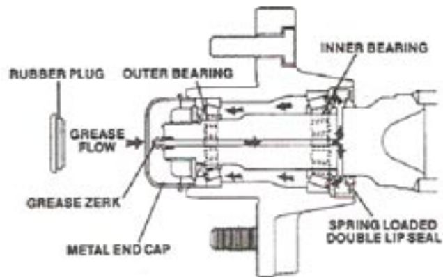
Figure 4: EZ-Lube Diagram
